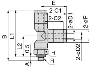
Metric thread
