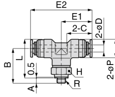
Metric thread
