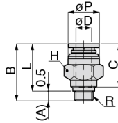
M5 Thread
