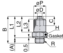
Metric thread
