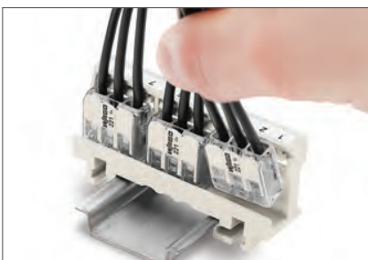
Install connectors into the mounting carrier
