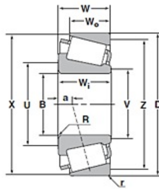
Tapered Roller Set - Inch Series and J Series - Dimensions
