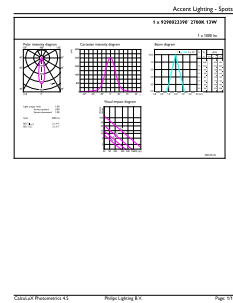
Accent Lighting Spots - MAS LEDspot D 13-100W E27 927 PAR38 25D
