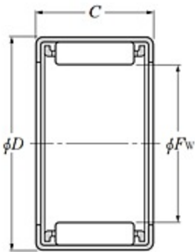
Drawn Cup Needle Roller Bearing - HK, HMK Type - Dimensions
