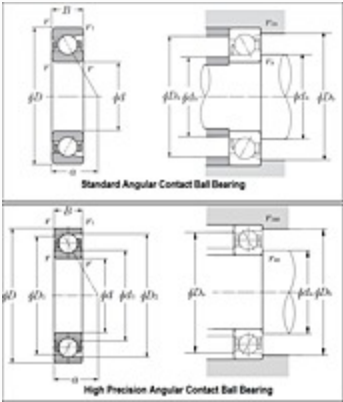
Single Angular Contact Ball Bearings - Open Type - Dimensions
