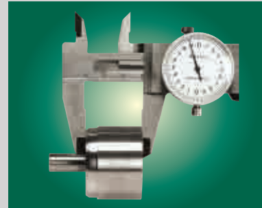
Outer diameter measurement
