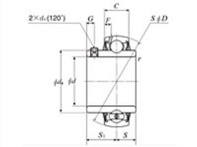
Bearing Insert w/ Set Screw, Wide Inner Ring - Spherical O.D. - Dimensions
