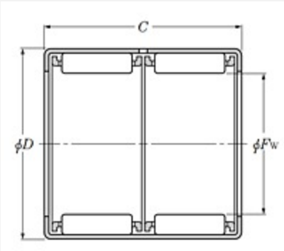
Drawn Cup Needle Roller Bearing - Double Row HK, HMK Type - Dimensions
