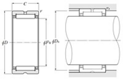
Machined-Ring Needle Roller Bearing w/o Inner Ring - RNA49.R, RNA59, RNA69.R, NK.R, MR Series - Dimensions
