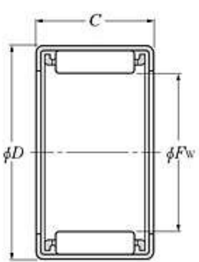
Drawn Cup Needle Roller Bearing - HK, HMK Type - Dimensions
