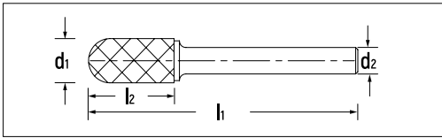
Dimension mark for carbide rotary file
