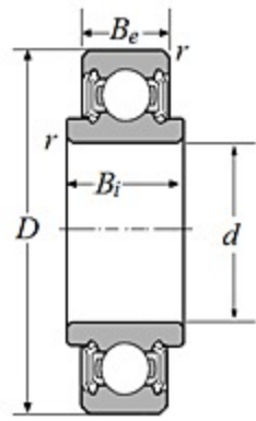
Single Row Radial Ball Bearing - Double Sealed (Contact Rubber Seal), 88000 Series - Dimensions
