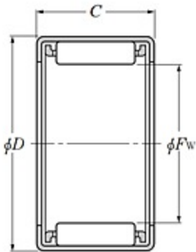
Drawn Cup Needle Roller Bearing - DCL Type - Dimensions
